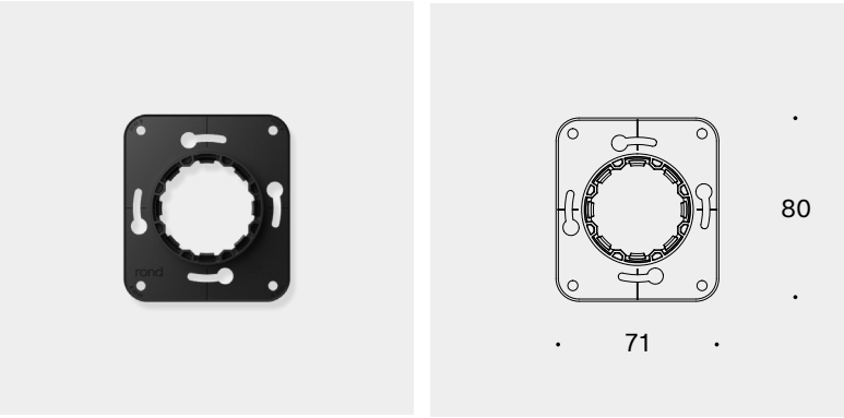
rond 3.0 | backfit holder
